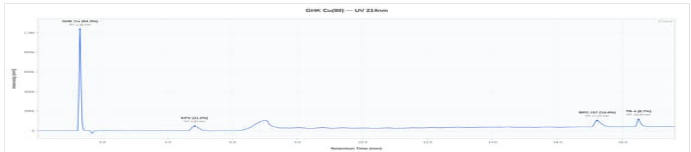
KLOW 80mg 80mg - EP-KLOW80-2: UV Chromatogram
